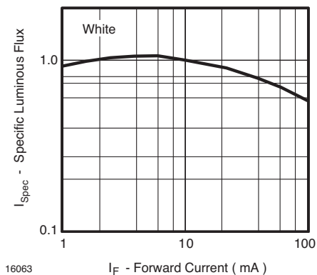
Figure 43. Specific Luminous Flux vs. Forward Current
