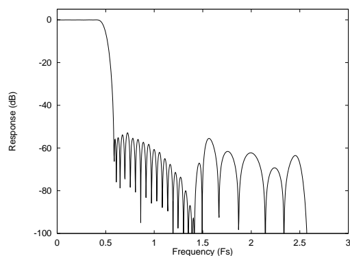
Figure 23 DAC Digital Filter Frequency Response – Type 0
