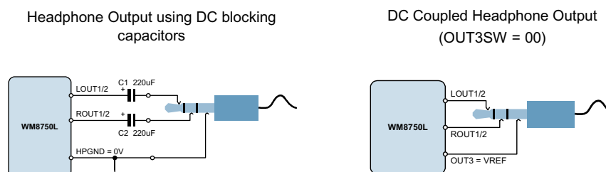
Figure 11 Recommended Headphone Output Configurations
