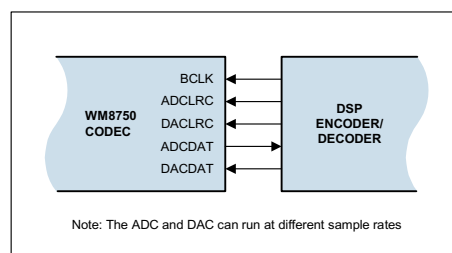
Figure 15 Slave Mode
