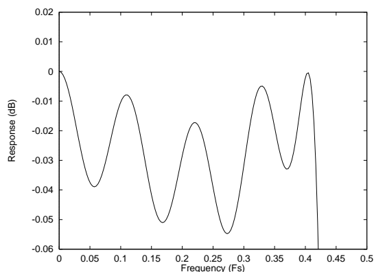
Figure 23 DAC Digital Filter Frequency Response – Type 0
