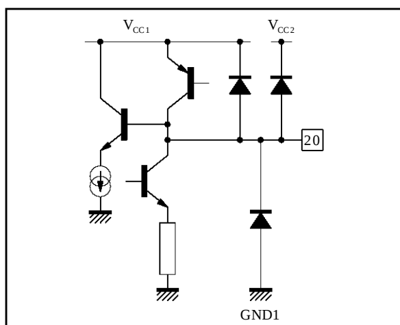
Figure 19 : Pin 20 - Y/CVBS
