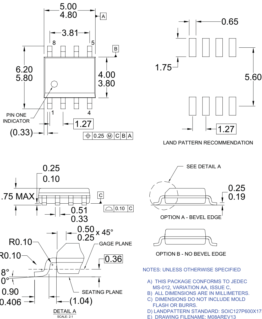
Figure 23. 8-Lead Small Outline Package (SOP)
