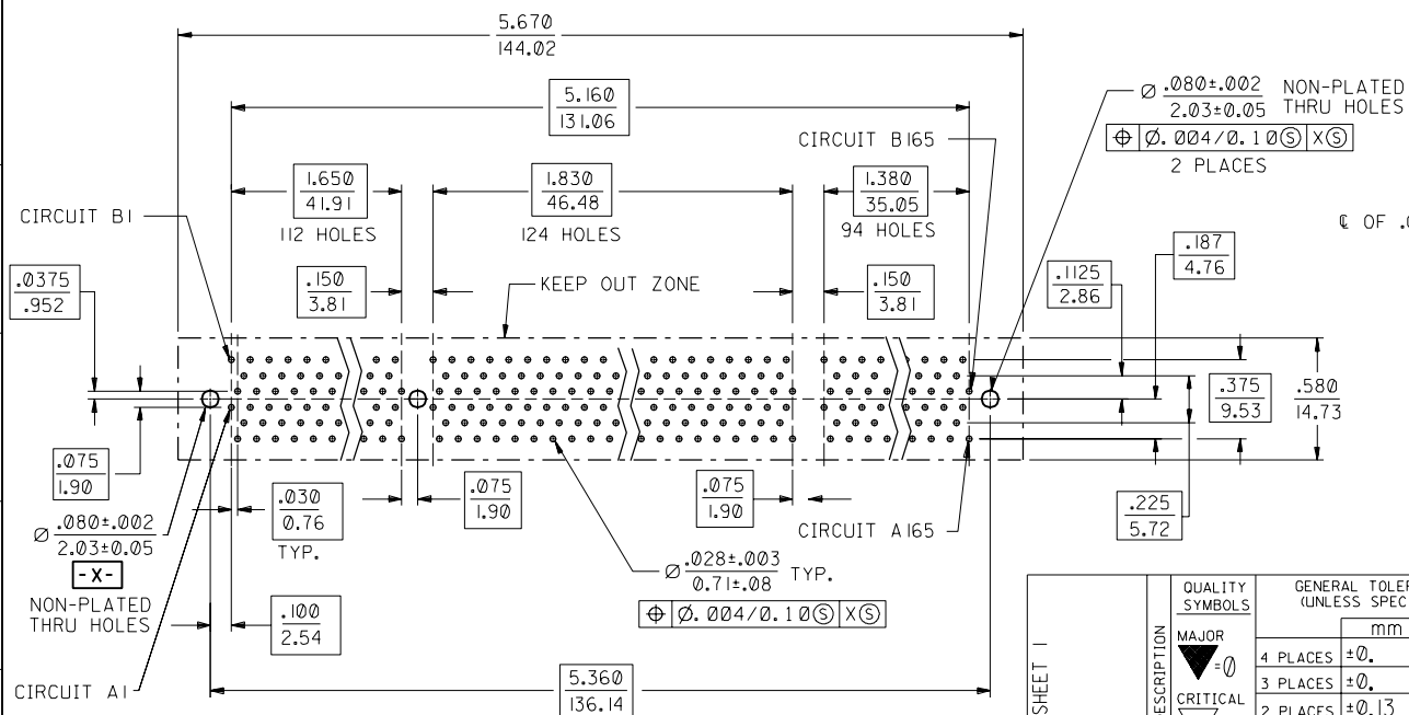
RECOMMENDED MODULE BOARD LAYOUT
