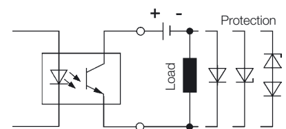
Protective circuit for DC output
