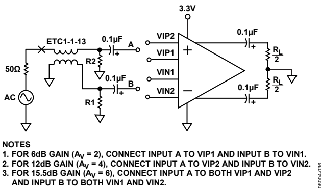
Figure 34. Differential-Input-to-Differential-Output Configuration
