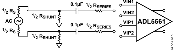
Figure 38. Gain Adjustment Using Series Resistor
