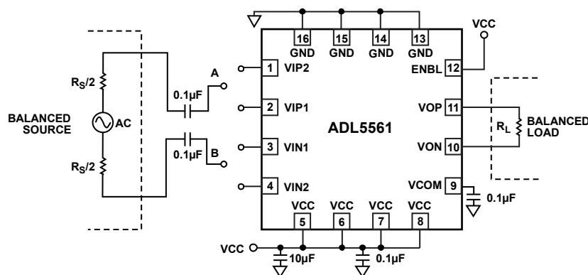
Figure 33. Basic Connections
