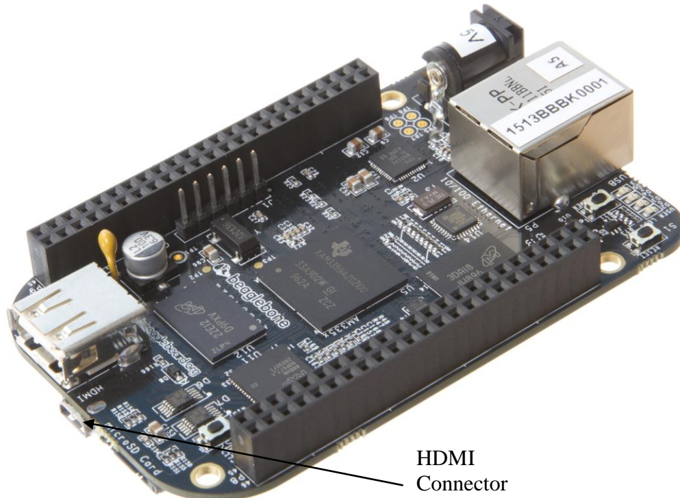
Figure 57. HDMI Connector
