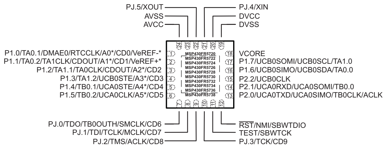
RGE PACKAGE (TOP VIEW)
