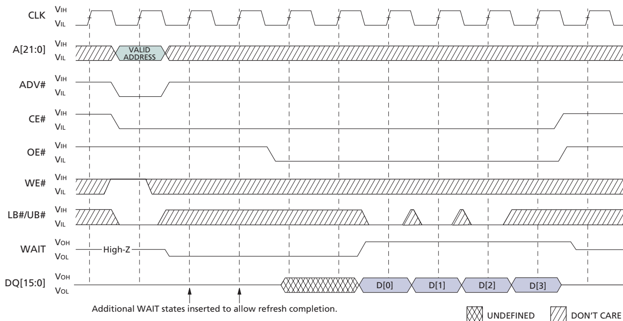
Figure 11: Refresh Collision During READ Operation
