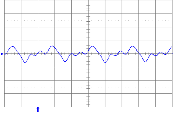
Fig. 1.5V.7: Output voltage ripple (20 mV/div.) at full rated load current into a resistive load with C_o = 10 \mu\text{F} tantalum + 1\mu\text{F} ceramic and V_{in} = 48 \text{ V} . Time scale: 1 \mu\text{s}/\text{div} .
