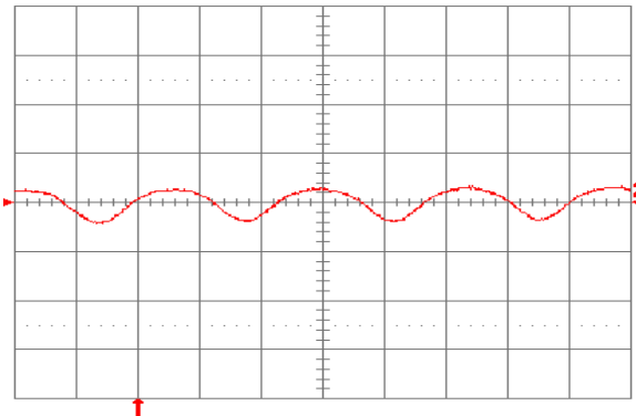
Fig. 1.2V.9: Input reflected ripple current, i_c (100 mA/div.), measured at input terminals at full rated load current and V_{in} = 48\ \text{V} . Refer to Fig. 1.2V.8 for test setup. Time scale: 1\ \mu\text{s}/\text{div} .
