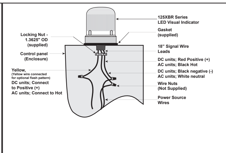
Figure 4. Panel Mounting
