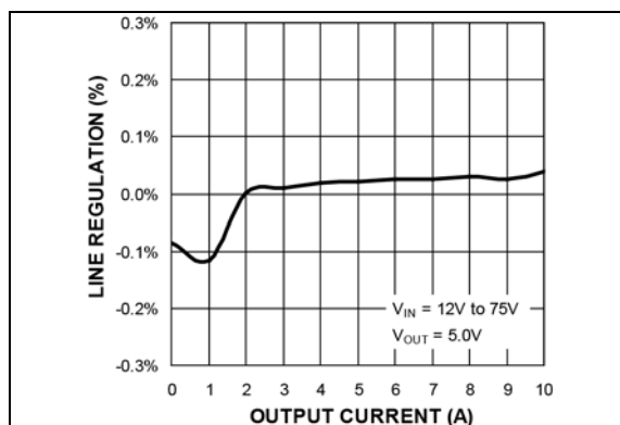
FIGURE 2-10: Line Regulation vs. Output Current (MIC2103).
