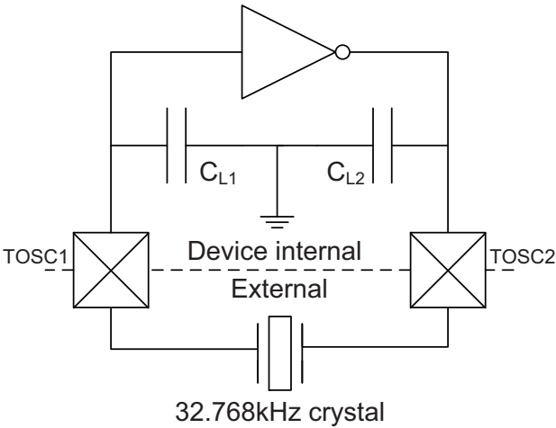
Figure 33-4. TOSC input capacitance.
