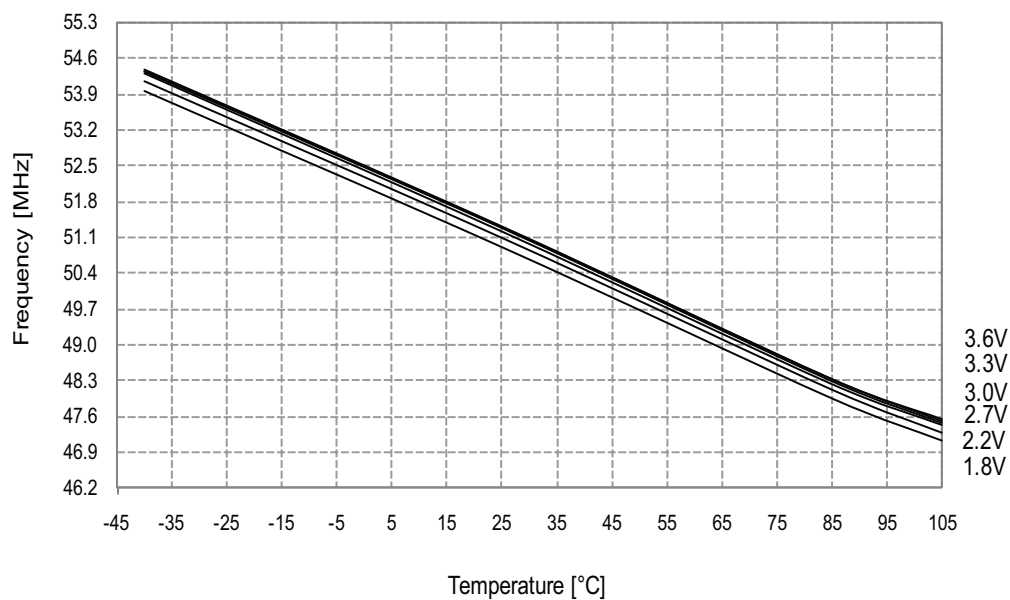
Figure 34-153. 48MHz internal oscillator frequency vs. temperature.
