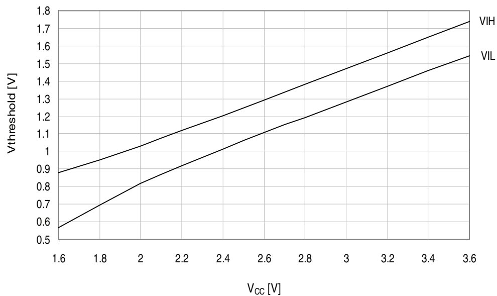
Figure 34-32. I/O pin input threshold voltage vs. V_{CC} . T = 25^\circ\text{C} .
