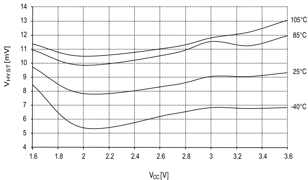
Figure 34-48. Analog comparator hysteresis vs. V_{CC} .
