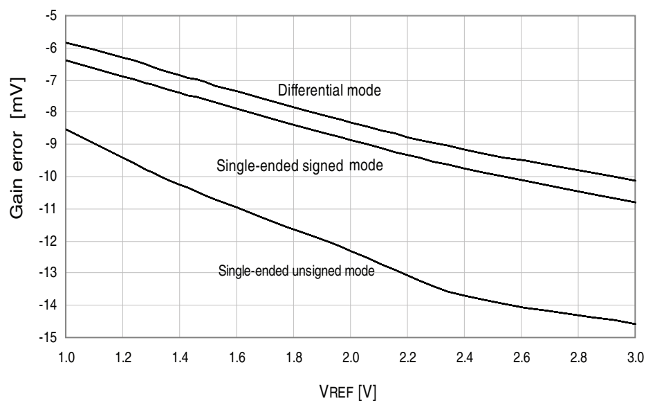
Figure 34-42. Gain error vs. V_{REF} .
