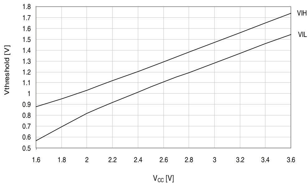
Figure 34-111. I/O pin input threshold voltage vs. V_{CC} . T = 25^\circ\text{C} .
