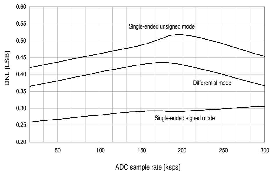
Figure 34-119. DNL error vs. sample rate. T = 25\text{ }^{\circ}\text{C} , V_{CC} = 3.6\text{V} , V_{REF} = 3.0\text{V} external.
