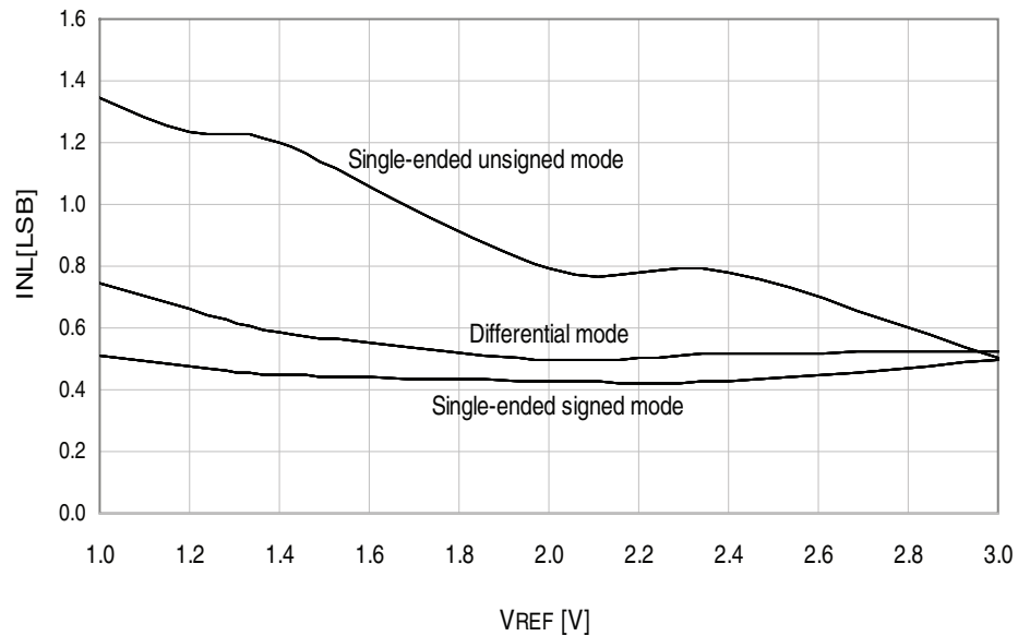
Figure 34-36. INL error vs. external V_{REF} .
