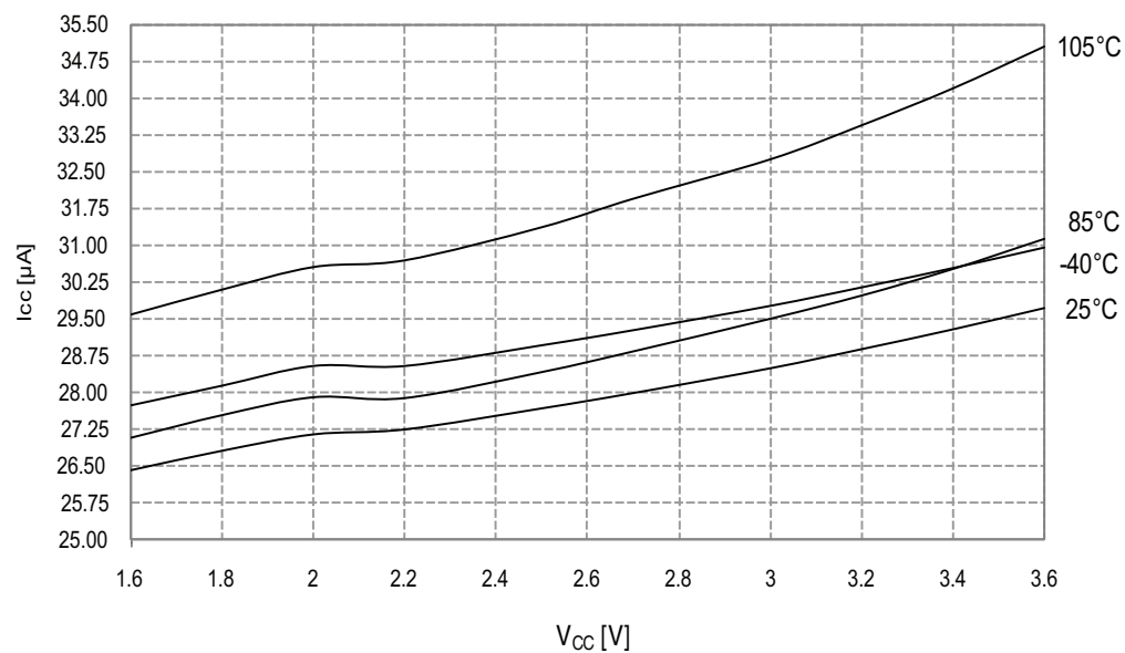
Figure 34-89. Idle mode supply current vs. V_{\text{CC}} .
