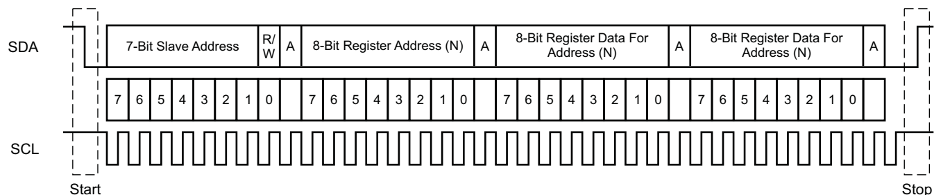
Figure 22. Typical I²C Sequence
