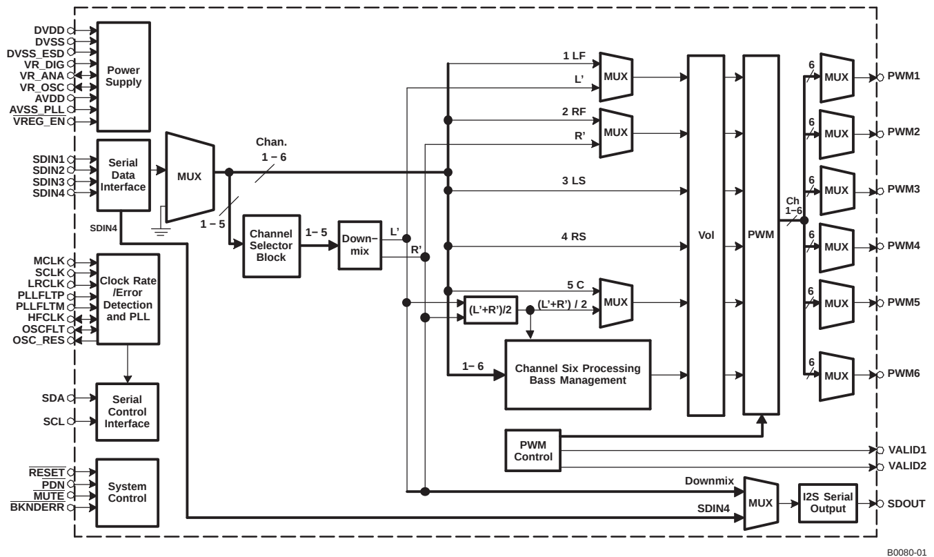
Figure 1. TAS5086 Functional Block Diagram
