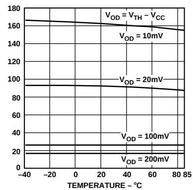
Figure 5. Power-Down RESET Delay vs. Temperature ADM8_T/S/R
