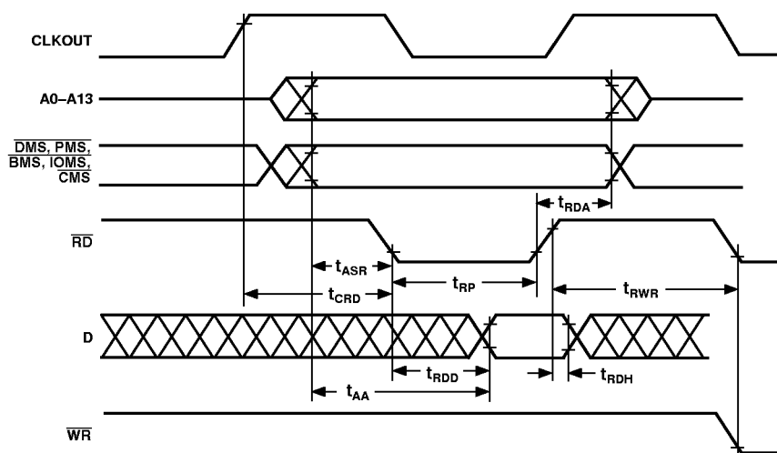
Figure 14. Memory Read
