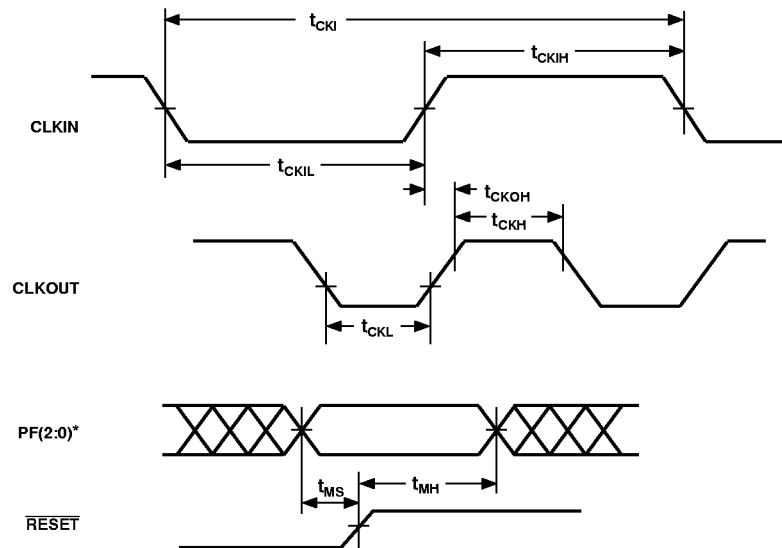
Figure 11. Clock Signals
