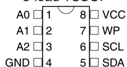
8-lead TSSOP
