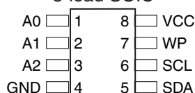
8-lead SOIC
