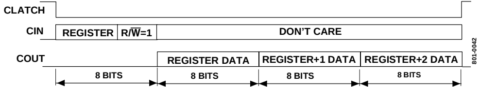
Figure 40. SPI Block Read Operation
