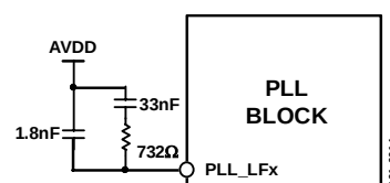
Figure 16. PLL L
