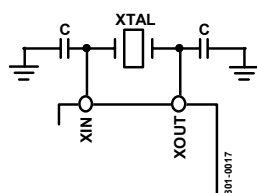
Figure 15. Crystal Connection
