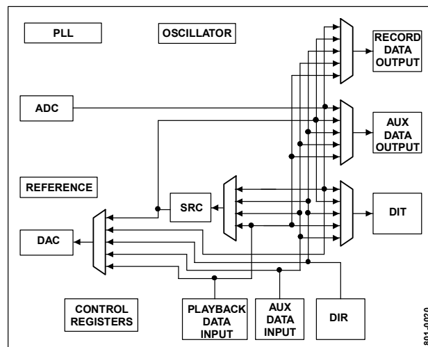
Figure 35. Data Path
