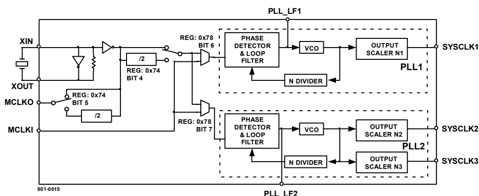
Figure 17. PLL Section Block Diagram
