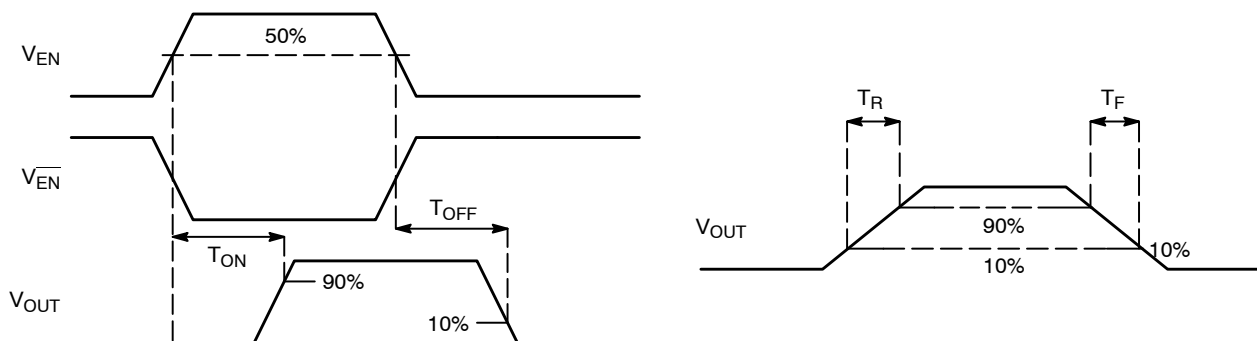
Figure 4. Voltage Waveform
