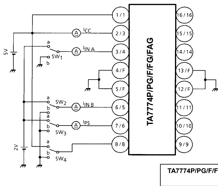
Test Circuit 1 I CC1 , I CC2 , I CC3 , I IN A , I IN B , I PS
