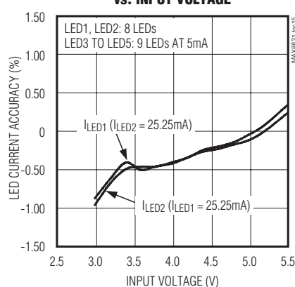
LED1, LED2 CURRENT ACCURACY vs. INPUT VOLTAGE MAX8831 ttc15
