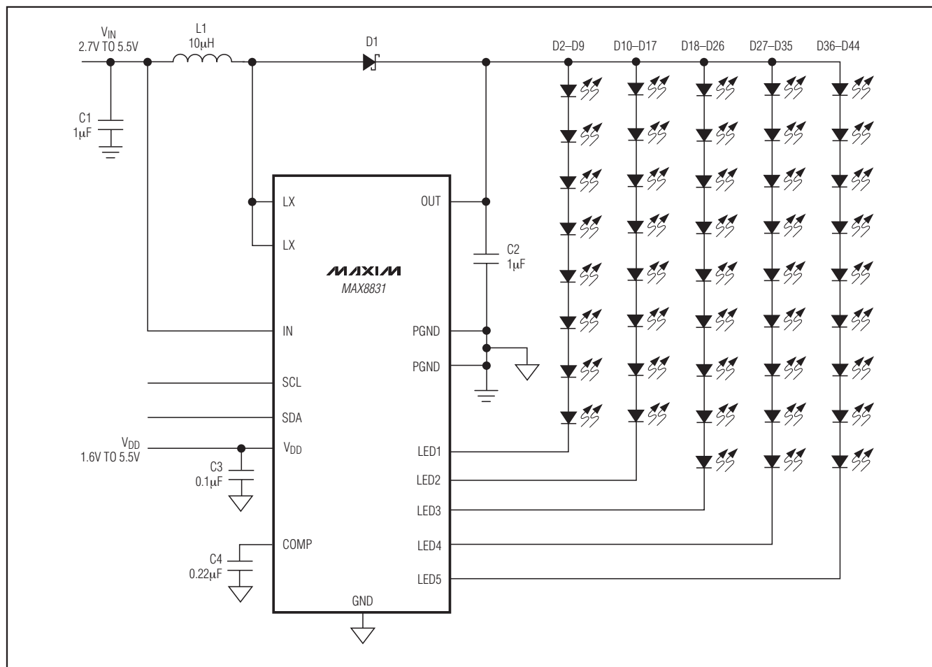
Figure 15. MAX8831 Applications Circuit
