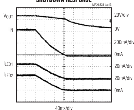
SHUTDOWN RESPONSE MAX8831 ttc13
