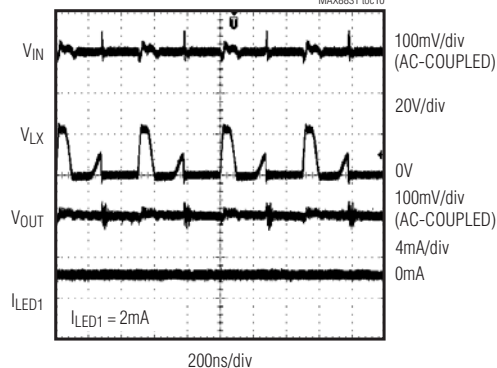
LIGHT-LOAD SWITCHING WAVEFORMS MAX8831 ttc10
