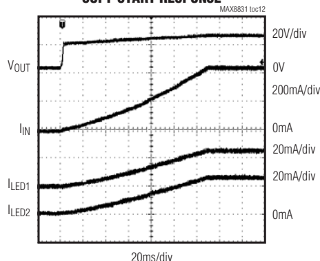
SOFT-START RESPONSE MAX8831 ttc12
