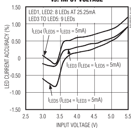
LED3-TO-LED5 CURRENT ACCURACY vs. INPUT VOLTAGE MAX8831 ttc16
