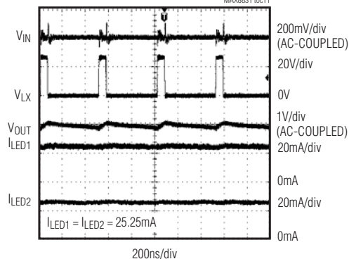
HEAVY-LOAD SWITCHING WAVEFORMS MAX8831 ttc11
