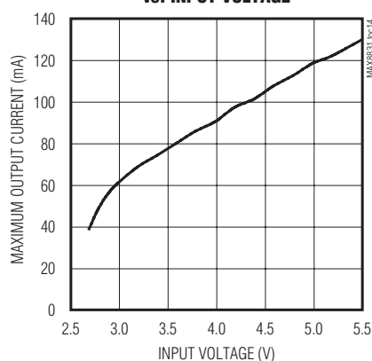
MAXIMUM OUTPUT CURRENT vs. INPUT VOLTAGE MAX8831 ttc14
