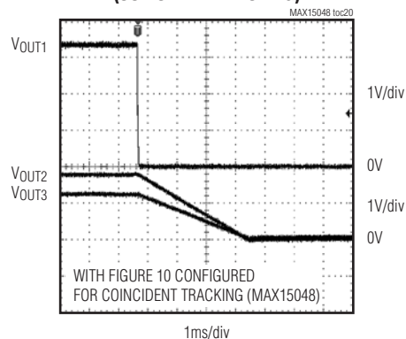
CHANNEL 1 SHORT CIRCUIT (COINCIDENT TRACKING)
