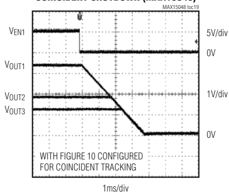
COINCIDENT SHUTDOWN (MAX15048)
