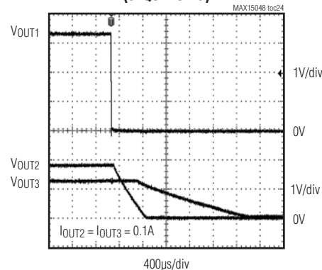
CHANNEL 1 SHORT CIRCUIT (SEQUENCING)
