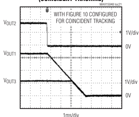
CHANNEL 2 SHORT CIRCUIT (COINCIDENT TRACKING)
