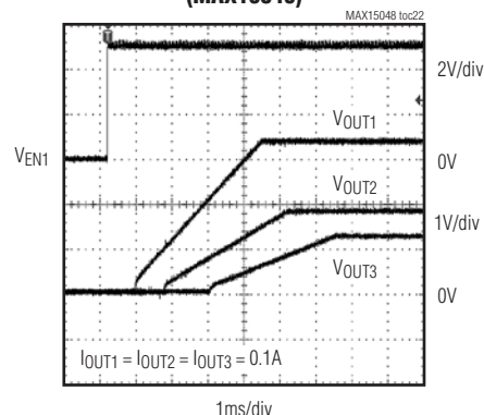
SEQUENCING STARTUP (MAX15049)
