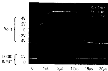
Output Waveform
