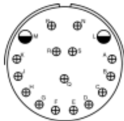
Insert Arrangement 36-13 Service Rating N, P, Q = E; Bal. = A Number of Contacts 2 15 Contact Size 12 16
