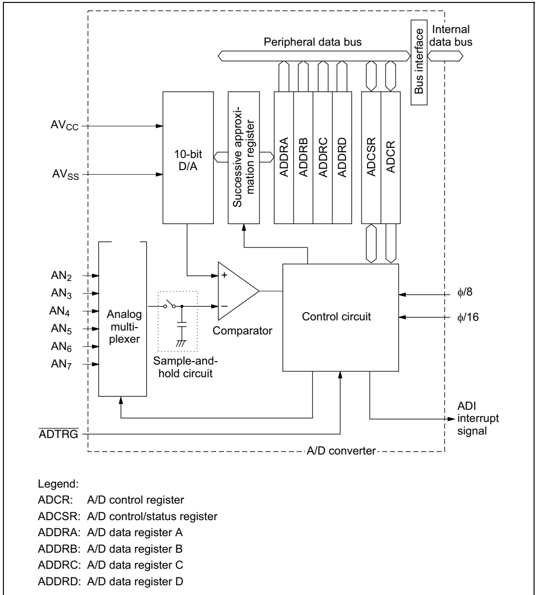
Figure 28.1 A/D Converter Block Diagram
