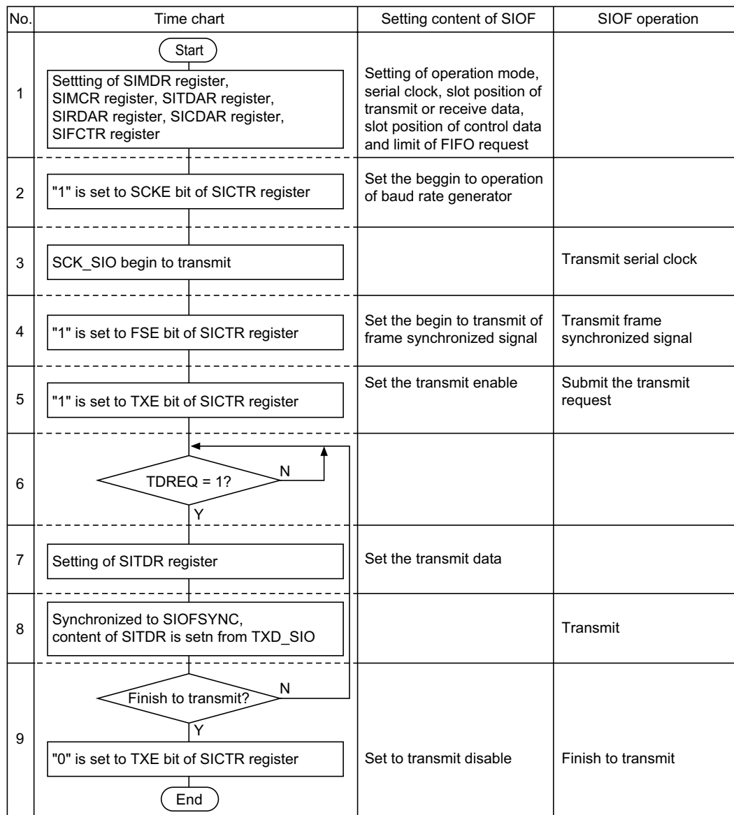
Figure 20.9 Example of Transmit Operation in Master
