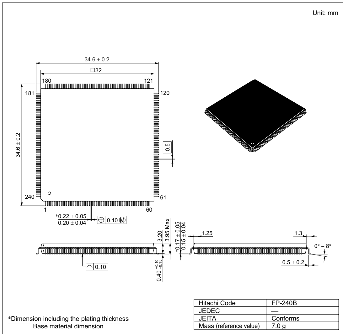
Figure D.1 Package Dimensions (FP-240B)
