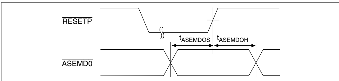
Figure 32.48 \overline{\text{ASEMDO}} Input Timing
