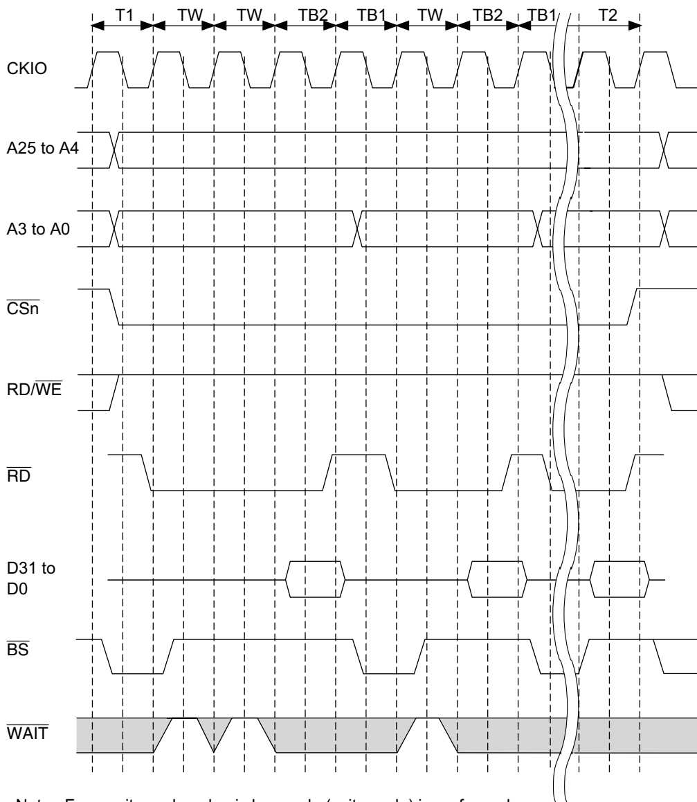
Figure 12.22 Burst ROM Wait Access Timing
