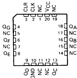
SN54HC4024 . . . FK PACKAGE (TOP VIEW)
