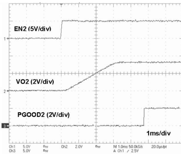
Figure 4-3. 3.3-V Start-Up Waveforms
