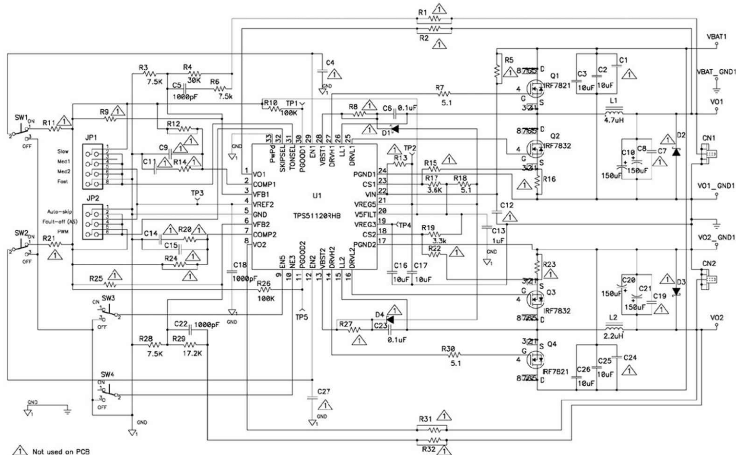
Figure 3-1. TPS51120 EVM Schematic Diagram
