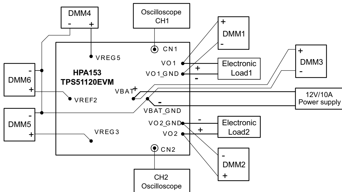
Figure 4-1. Equipment Setup for TPS51120EVM-001 Board
