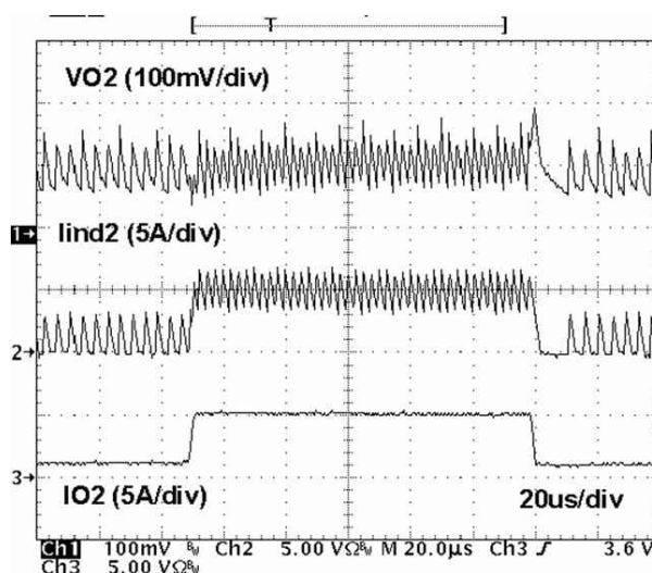
Figure 4-5. 3.3-V Load Transient Response
