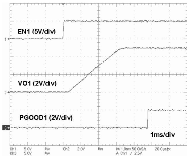
Figure 4-2. 5-V Start-Up Waveforms
