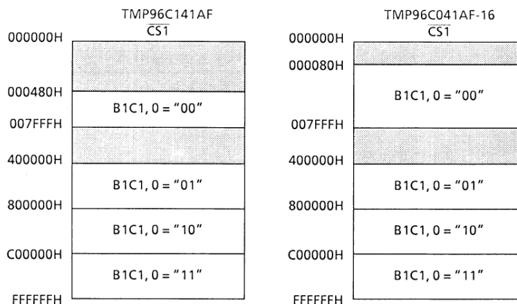
Fig. 3.2 (2). \overline{\text{CS1}} Address Area
