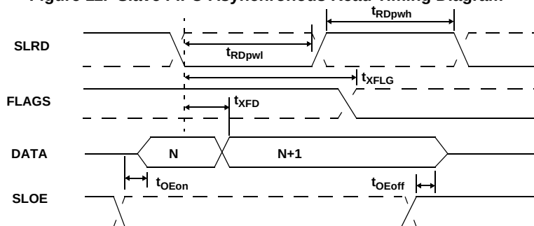
Figure 11. Slave FIFO Asynchronous Read Timing Diagram [19]
