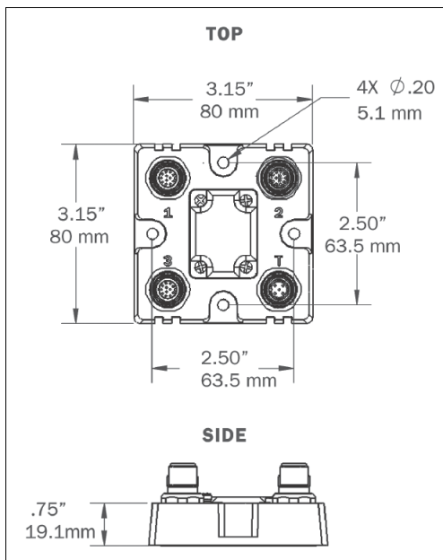
QX-1 Dimensions
