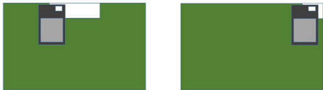
Figure 6.1. Recommended Application PCB Layout for the BGM113 Module
