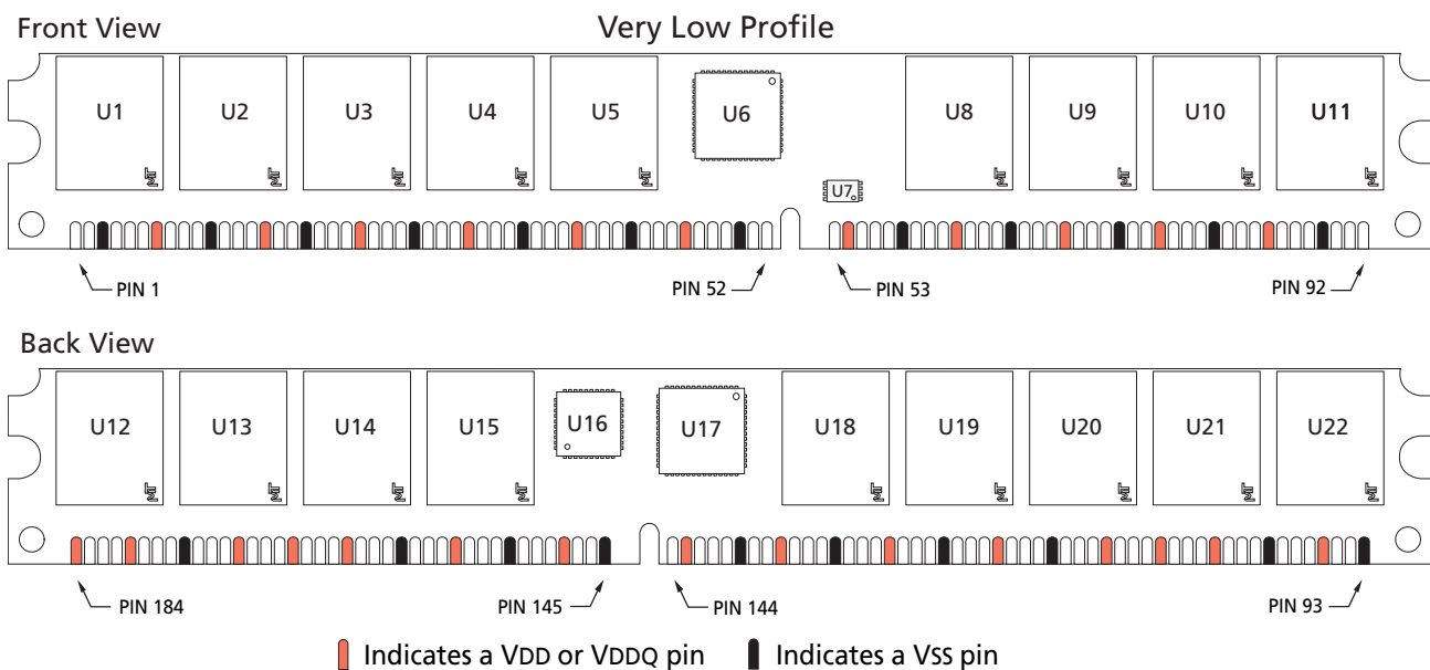
Figure 2: Pin Locations
