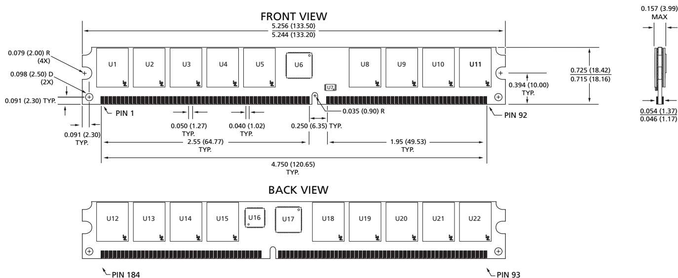
Figure 16: 184-Pin VLP RDIMM Dimensions
