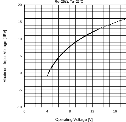
Maximum Input Voltage vs. Operating Voltage (BYPASS)
