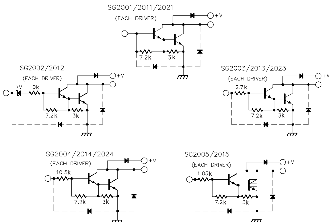
Figure 1 · Partial Schematics
