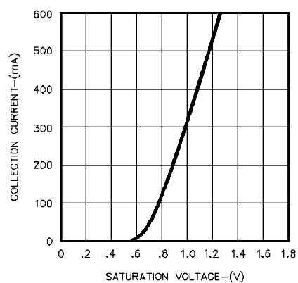
FIGURE 2. OUTPUT CHARACTERISTICS
