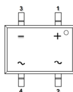
Pin Diagram
