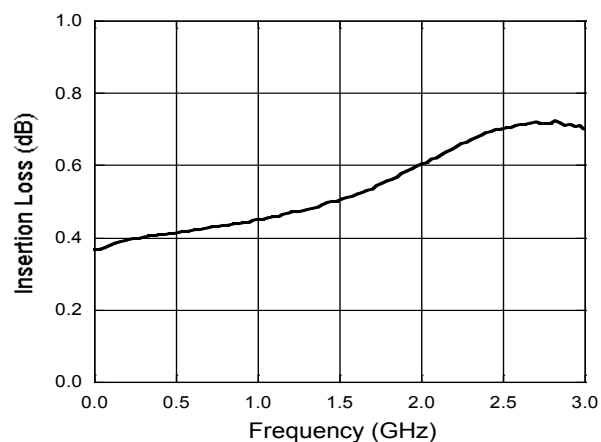
Insertion Loss
