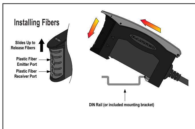
Figure 2. Installing D10 fibers and housing
