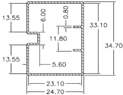
Profile view
