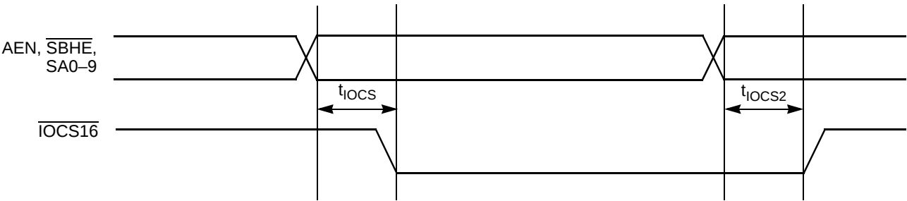
\overline{\text{IOCS16}} Timings
