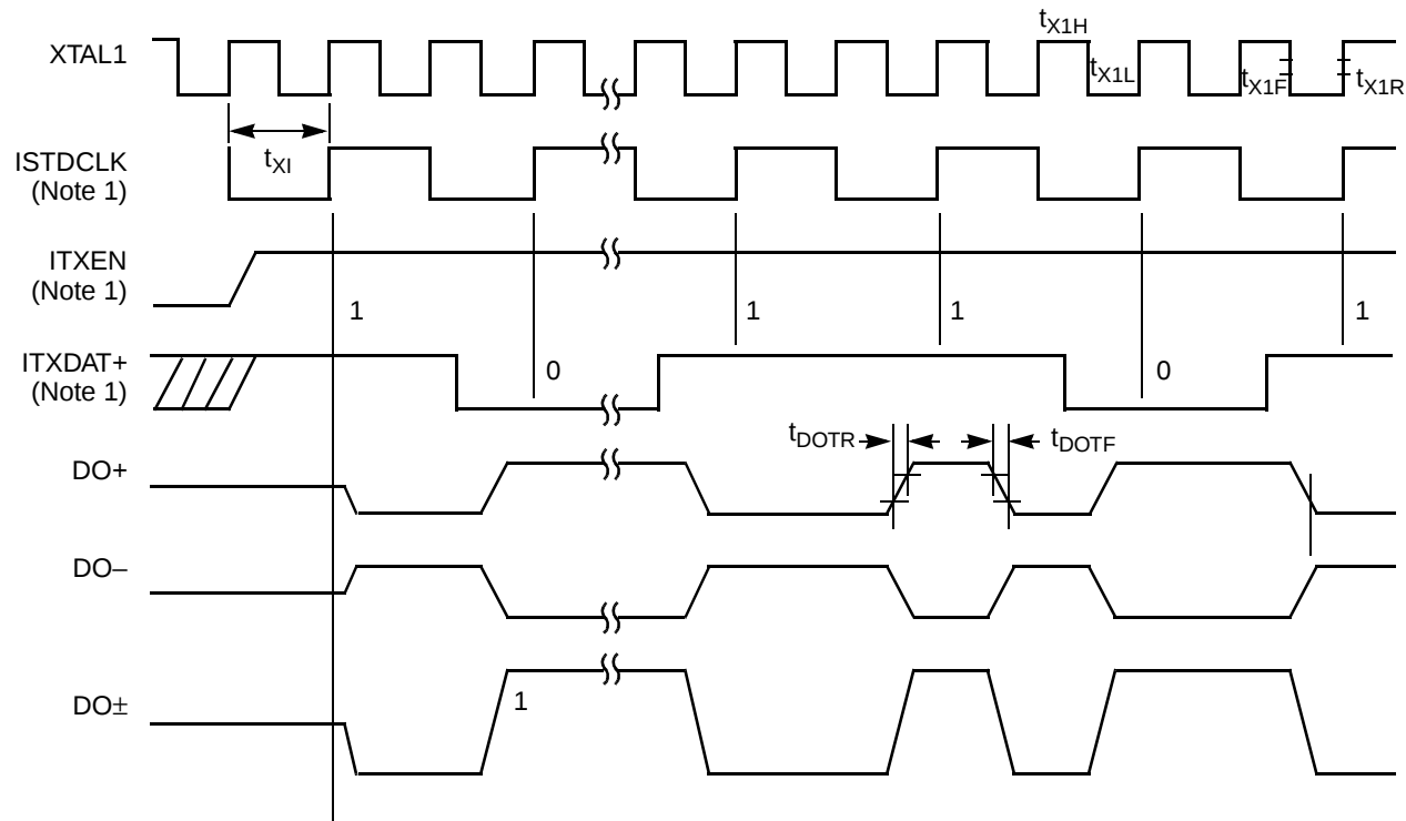
Transmit Timing—Start of Packet
