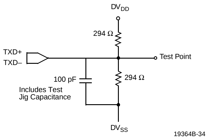
TXD Switching Test Circuit
