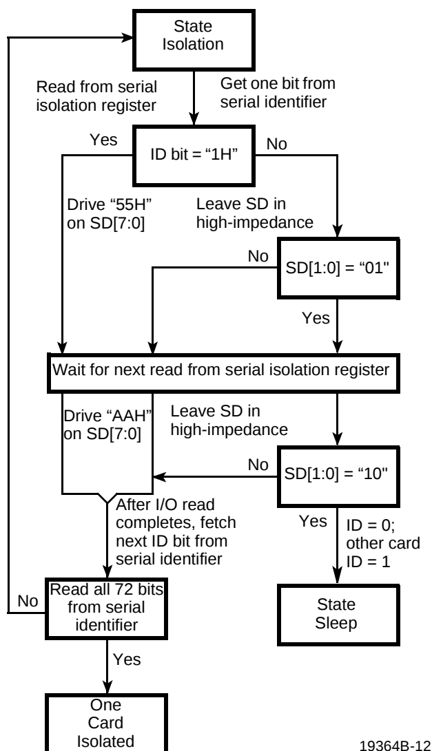
Plug and Play ISA Card Isolation Algorithm
