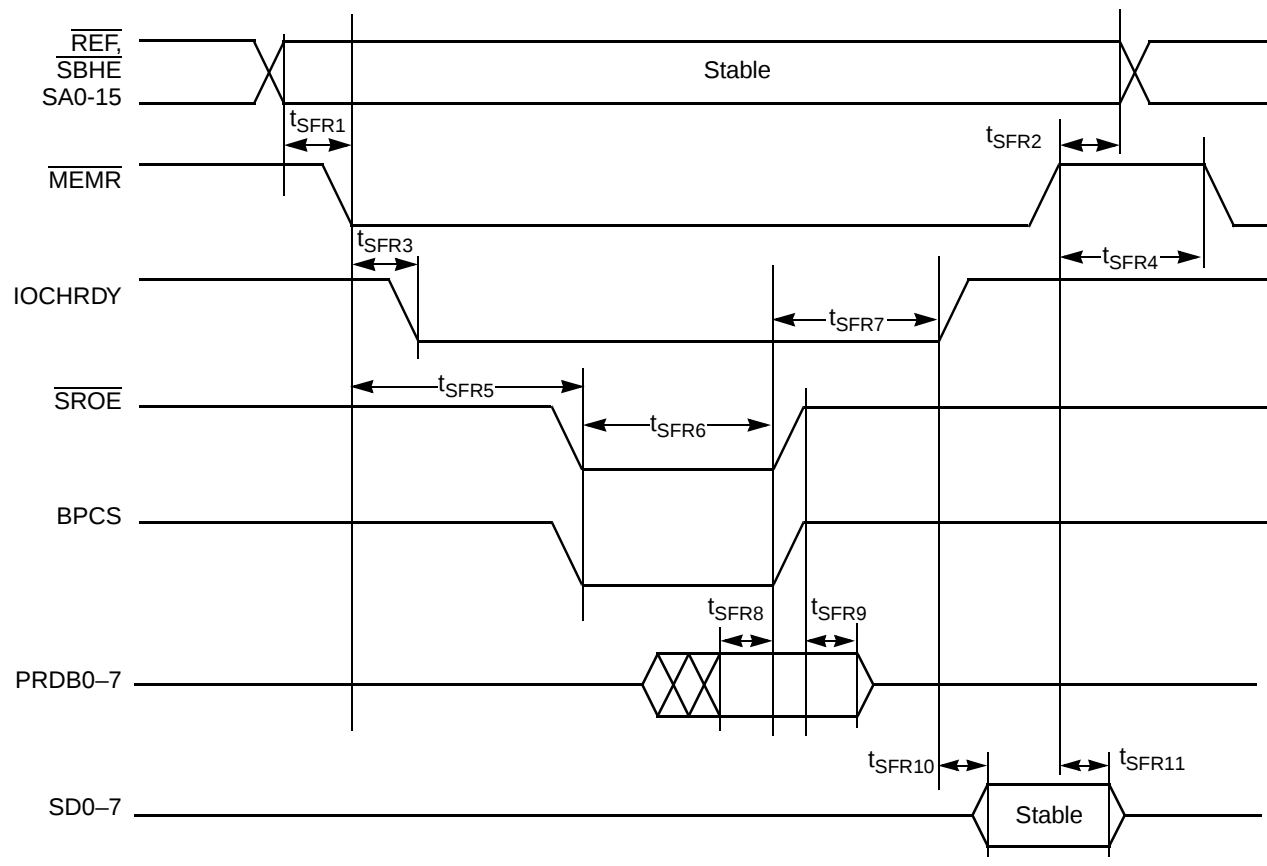
Flash Read Cycle 19364B-64
