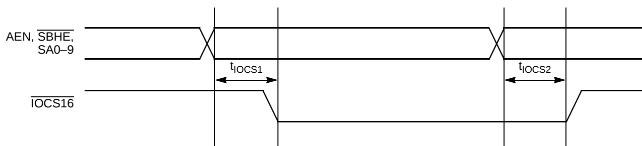
\overline{I/OCS16} Timings
