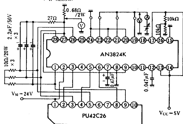
Test Circuit 5 ( V_{H-OFFSET} )
