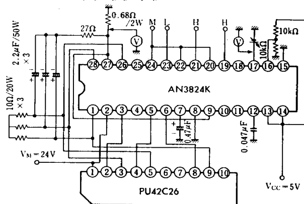
Test Circuit 4 ( V_{H-ALLOW} )
