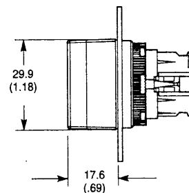
Illuminated Push Button, Flush
