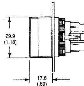
Non-Illuminated Push Button, Extended
