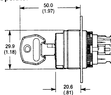
Key Operated Selector Switch Operator
