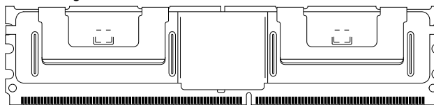
Figure 1: 240-Pin FBDIMM (MO-256 R/C A)
