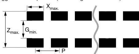
Suggested land pattern (according to IPC-7351A)
