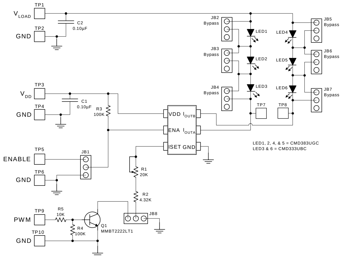
Figure 2 – Schematic
