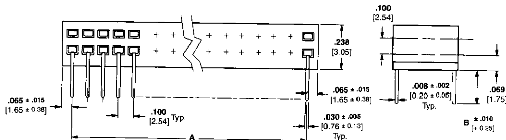
Housing Configuration 1
