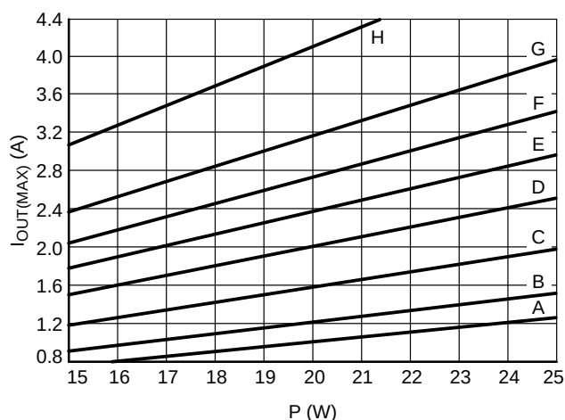
Figure 19. Current Limit Characteristics
