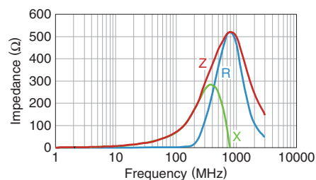
MMZ1005D680C
