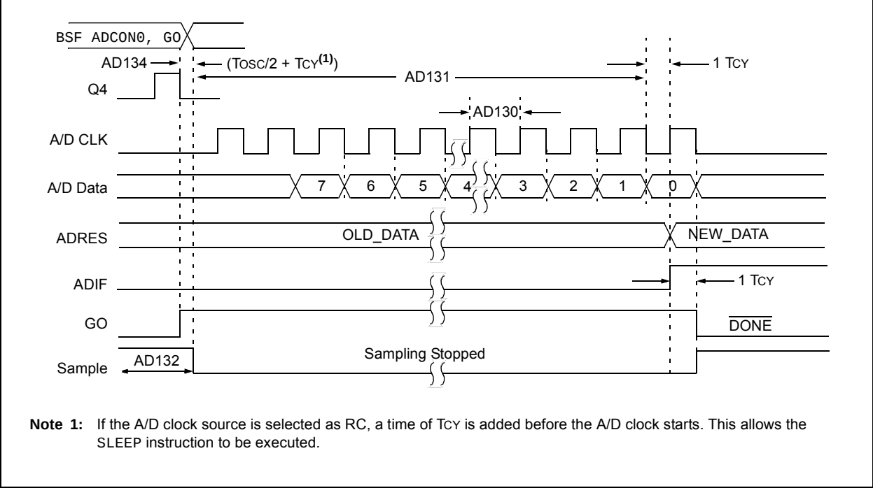
FIGURE 30-13: PIC16(L)F1934/6/7 A/D CONVERSION TIMING (SLEEP MODE)
