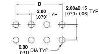
Recommended Solder Pad Layout
